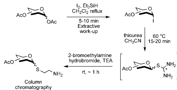
Scheme 2. One-Pot Sequence for Thioglycoamine Formation a
