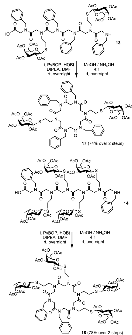
Scheme 4. Macrocyclization Reaction and Global Deprotection
