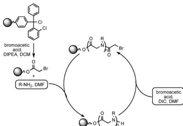
Scheme 1. Sub-monomer Peptoid Solid-Phase Strategy on a Trityl Resin
