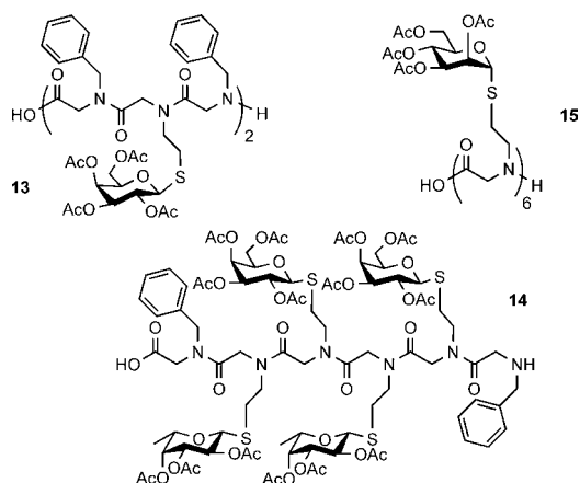
Figure 1. Linear S-linked glycopeptoids.
