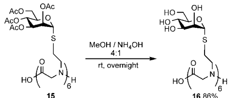
Scheme 3. Deprotection of Hexamannopeptoid 15
